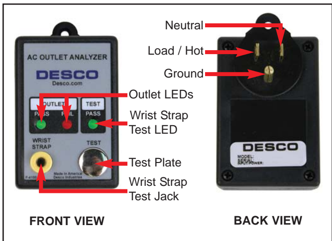
Figure 3. 98130 120V AC Outlet Analyzer and Wrist Strap Tester features and components
